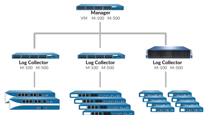
Figure 3: Panorama Architecture
