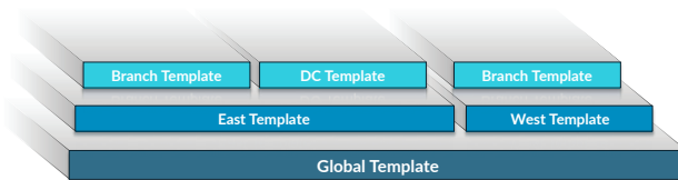
Figure 3: Template Stacking
